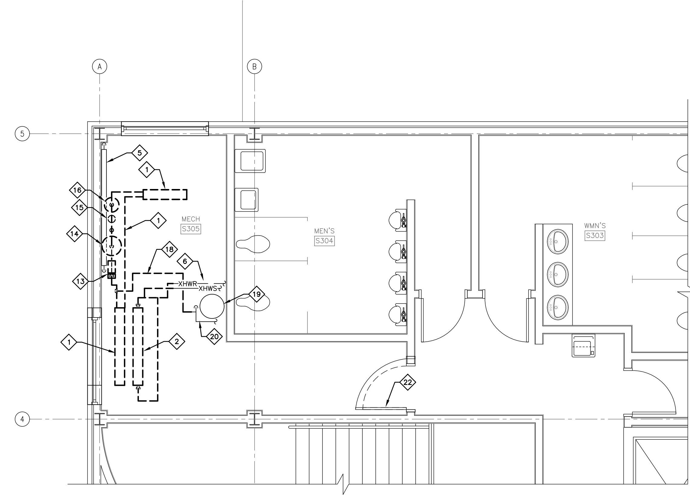
THIRD FLOOR PART PLAN – PIPING DEMOLITION SCALE: 1/4" = 1'-0"
