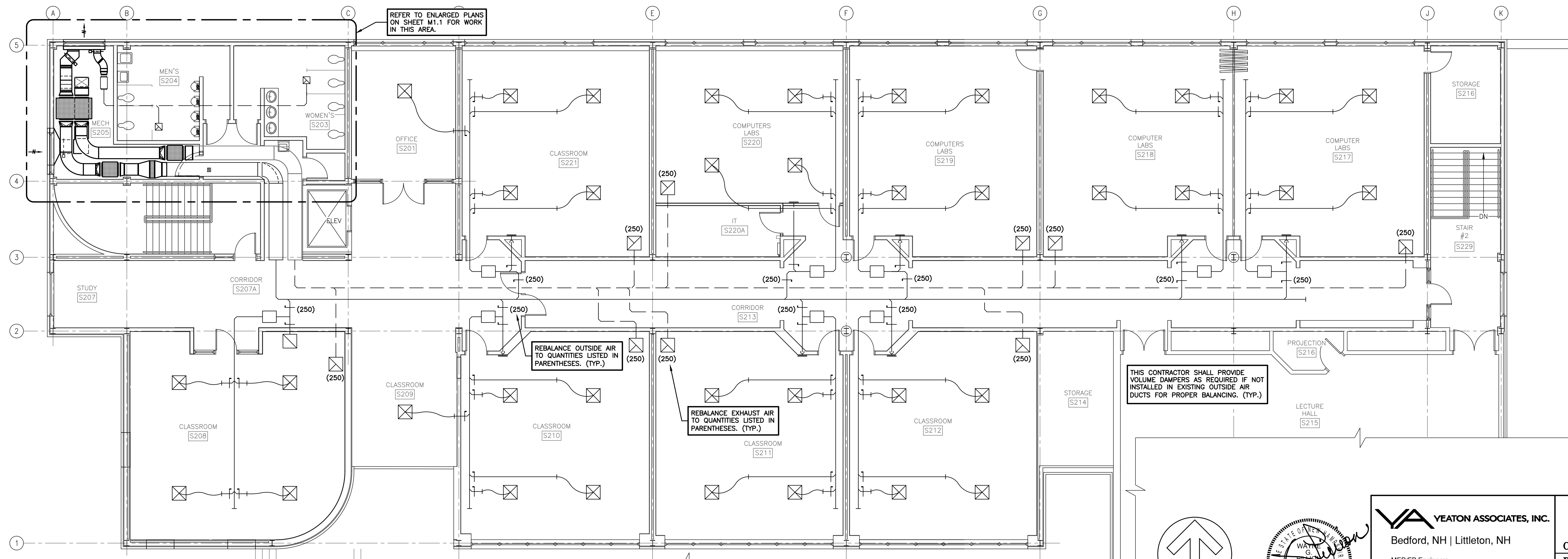
SECOND FLOOR PART PLAN - DUCTWORK
