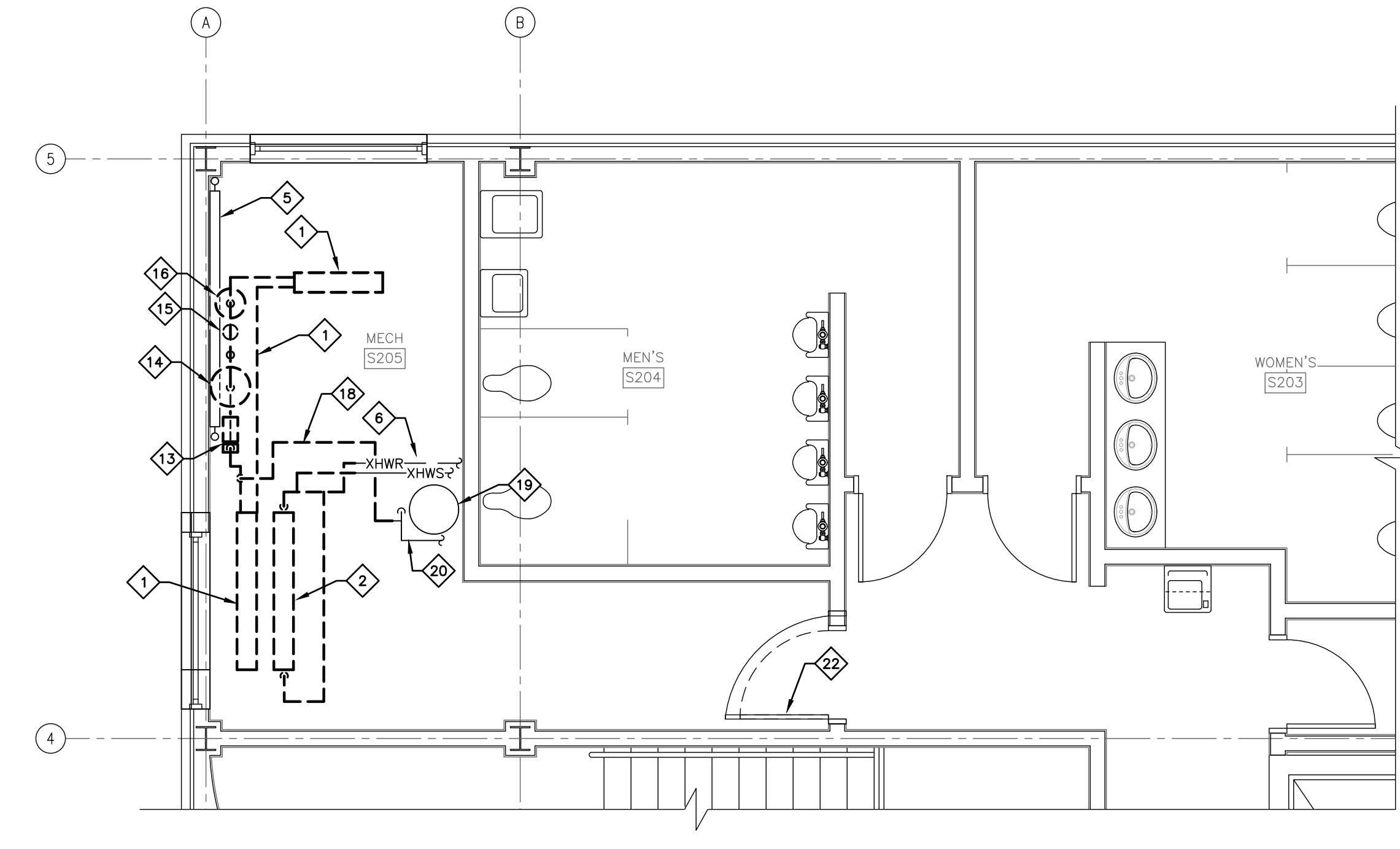
SECOND FLOOR PART PLAN – PIPING DEMOLITION SCALE: 1/4" = 1'-0"
