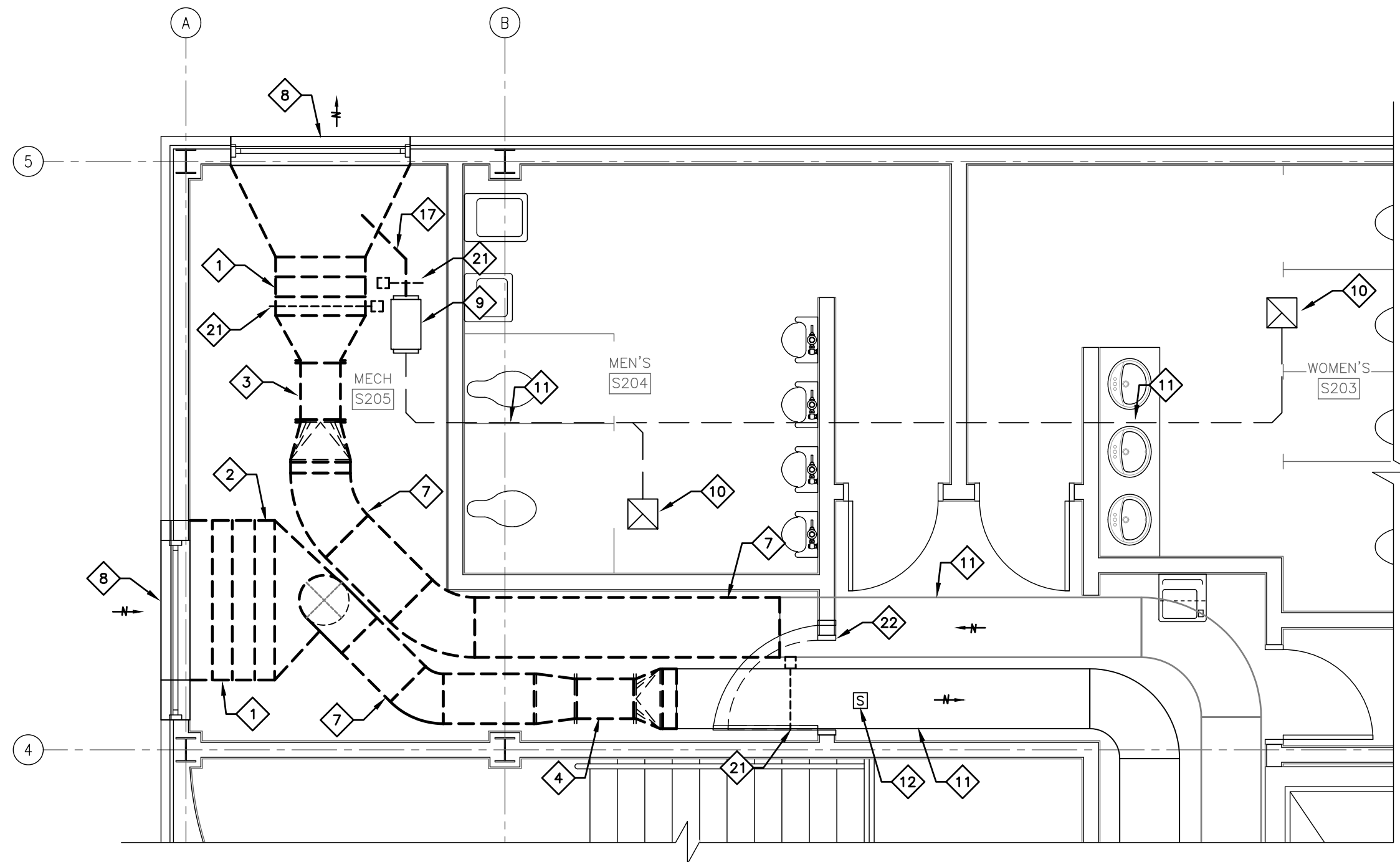
SECOND FLOOR PART PLAN – DUCTWORK DEMOLITION SCALE: 1/4" = 1'-0"
