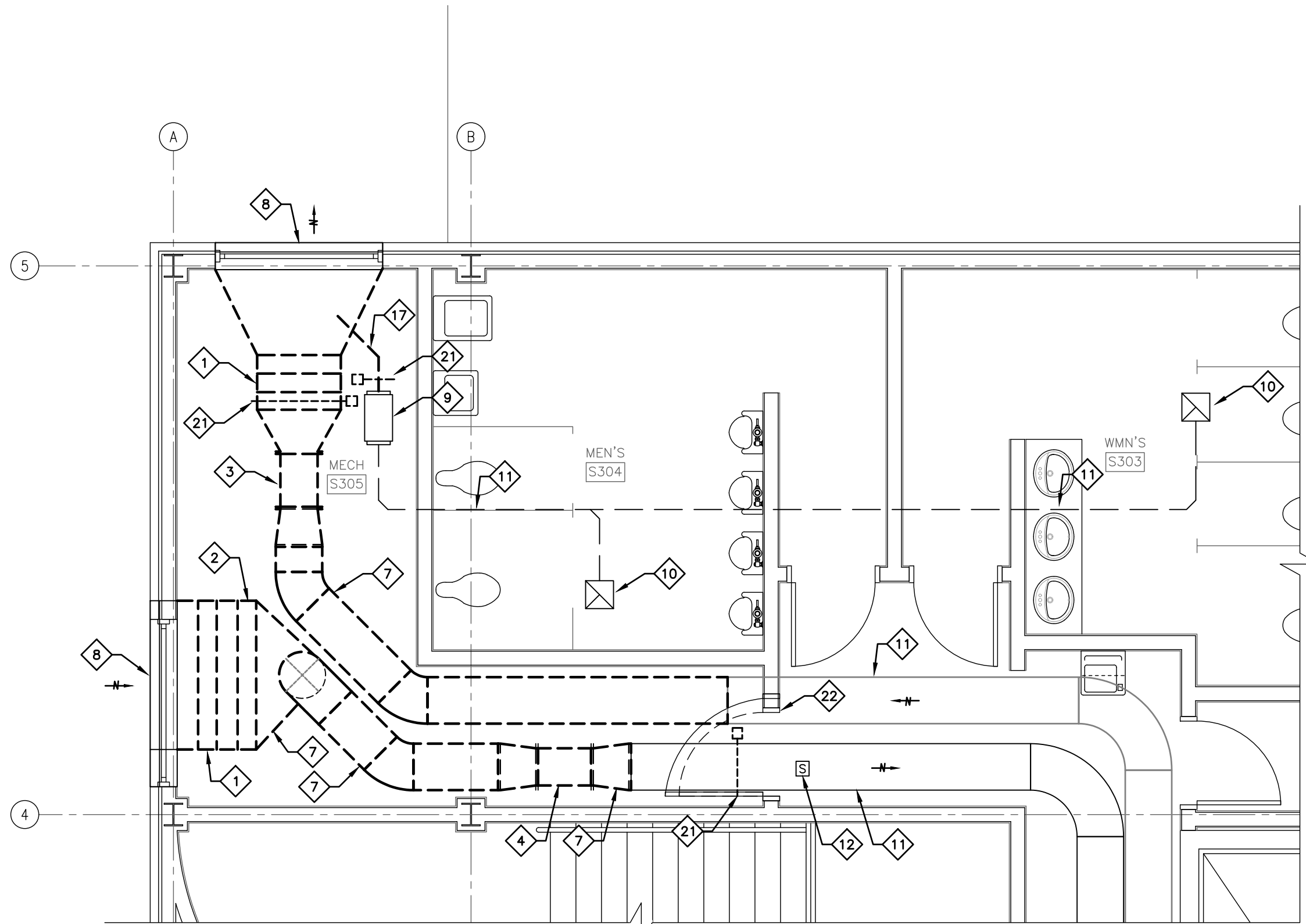
THIRD FLOOR PART PLAN – DUCTWORK DEMOLITION SCALE: 1/4" = 1'-0"
