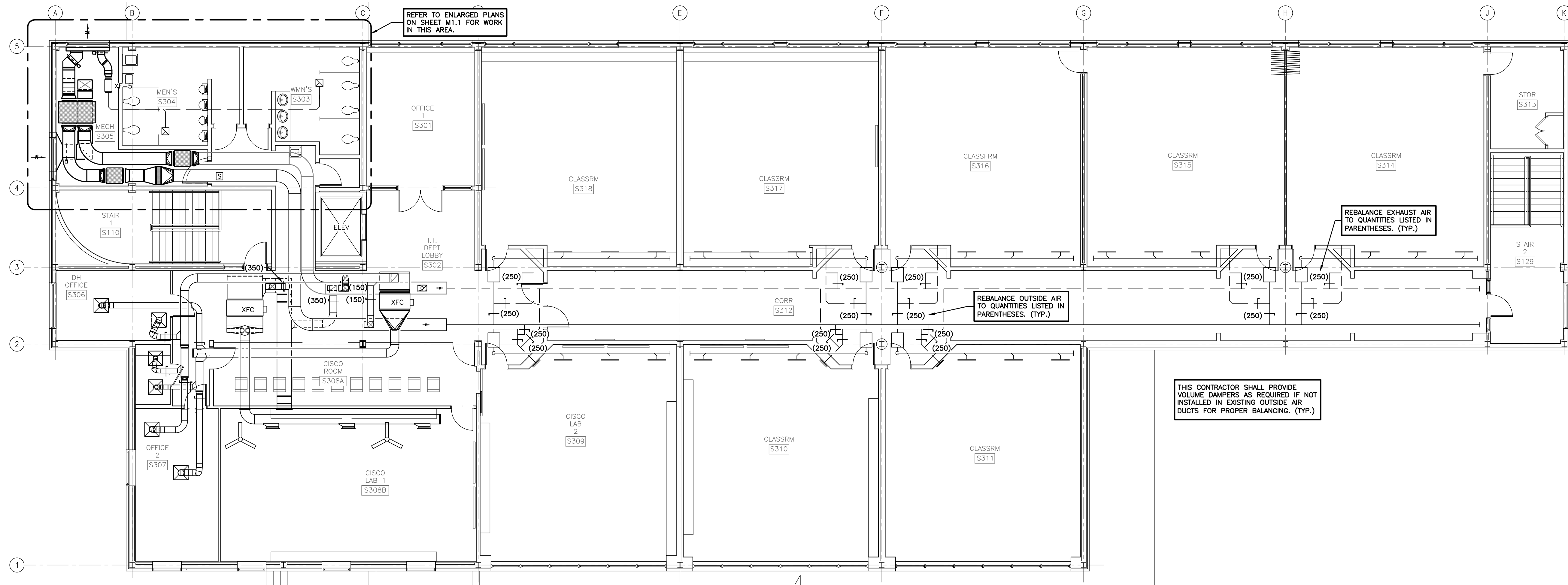
THIRD FLOOR PART PLAN - DUCTWORK
